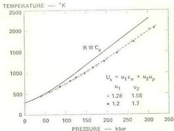
FIG. 5. Shock temperature for water. Comparison of the constant C_v model with the Rice-Walsh constant C_p model. The shock temperatures calculated using the constant C_v model are not sensitive to the form of the Hugoniot. u_1, u_2 = 1.28, 1.58 (personal communication from R. W. Woolfolk); 1.2, 1.7 (Ref. 3). The other input data are in Table I.
